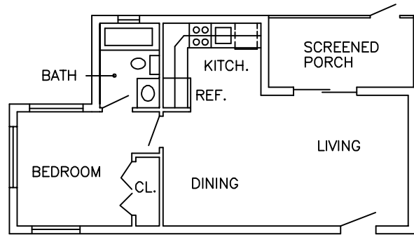
UNIT 5 (UNIT 6 = MIRROR IMAGE)
