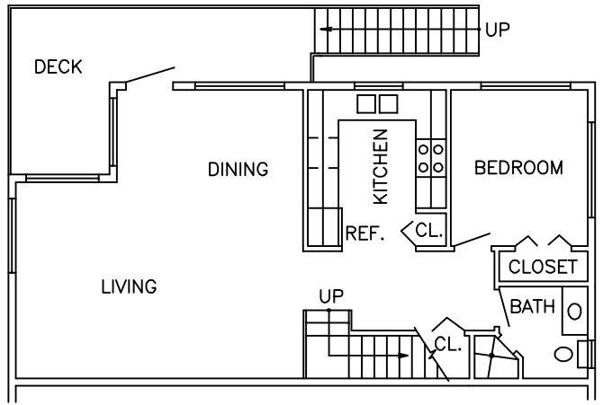
UNIT B & F LOWER LEVEL (UNIT C MIRROR IMAGE)
